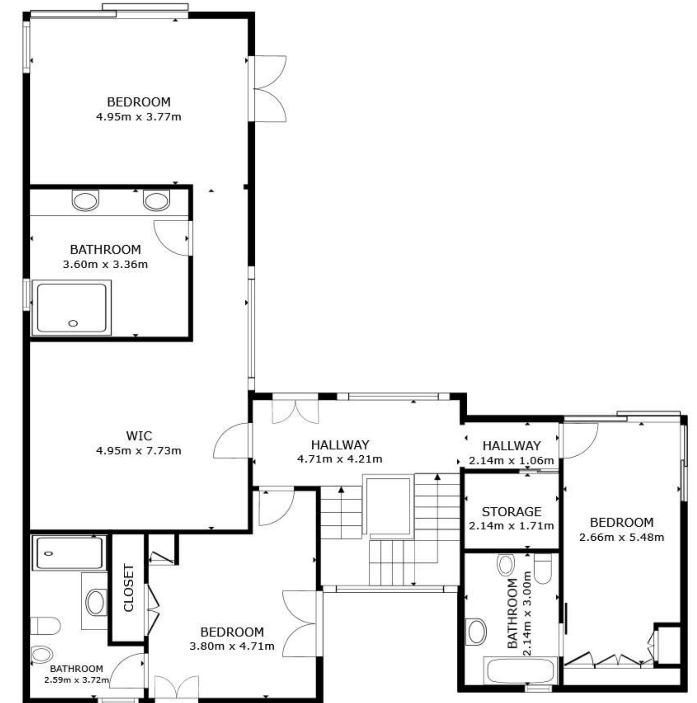
FLOOR 3
